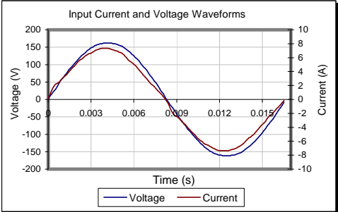
Input AC Current Waveform (ITHD = 3.83%, 50% Load)
