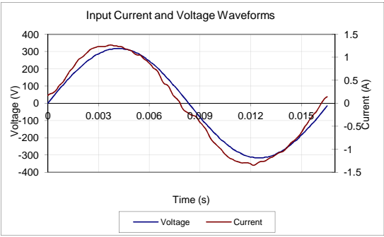
Input AC Current Waveform (ITHD = 5.09%, 50% Load)
