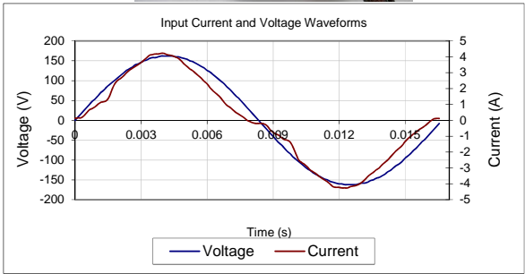
Input AC Current Waveform (ITHD = 16.7%, 50% Load)
